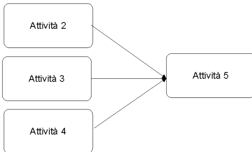
Fig. 4.11: Or-split.
